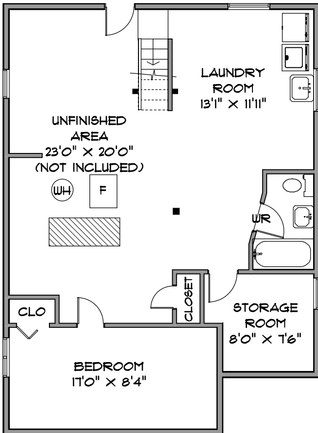
LOWER LEVEL 508 SQ.FT.
