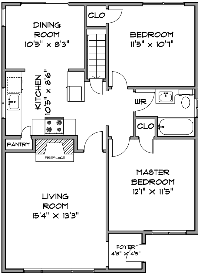
MAIN LEVEL 895 SQ.FT.
